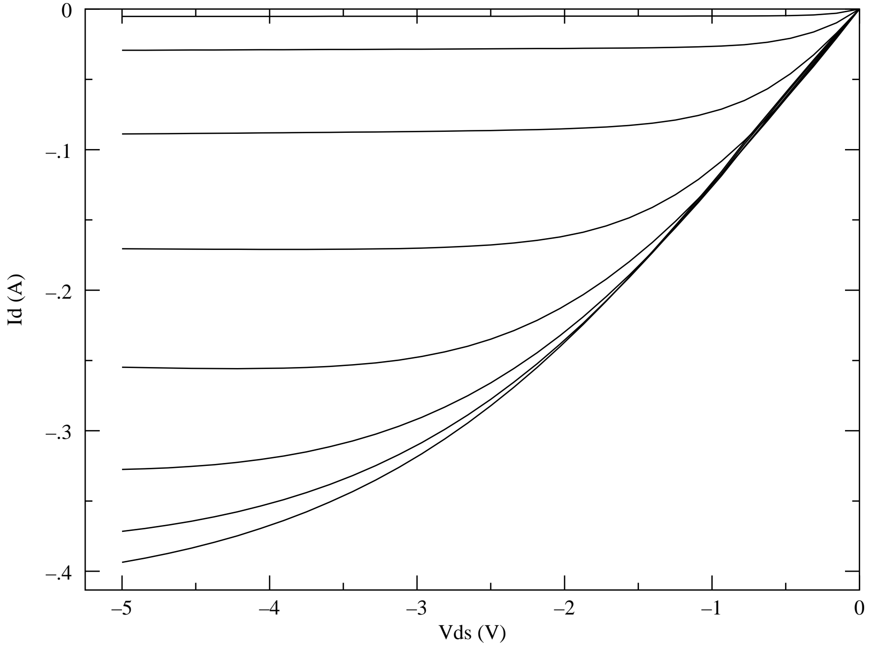
Characteristic Curves for pMOSFET
