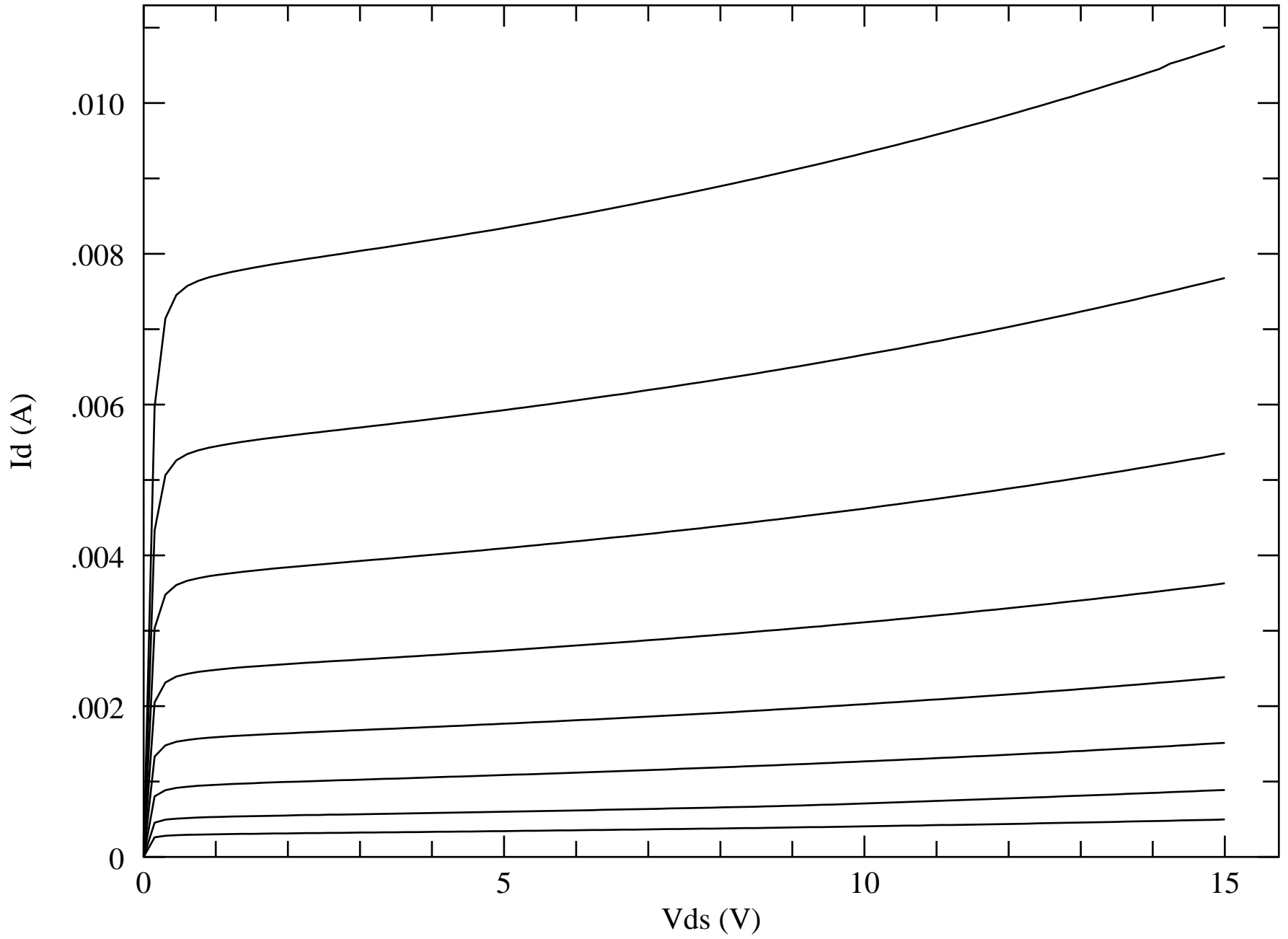
Characteristic Curves for nMOSFET
