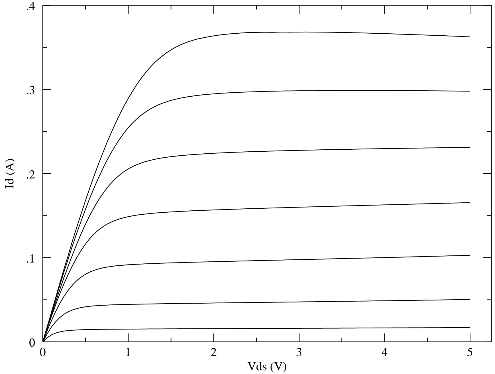
Characteristic Curves for nMOSFET
