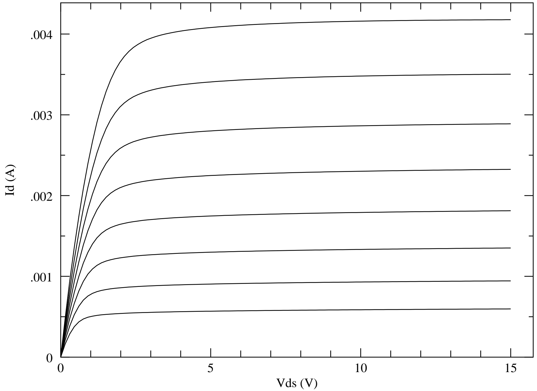
Characteristic Curves for nFET
