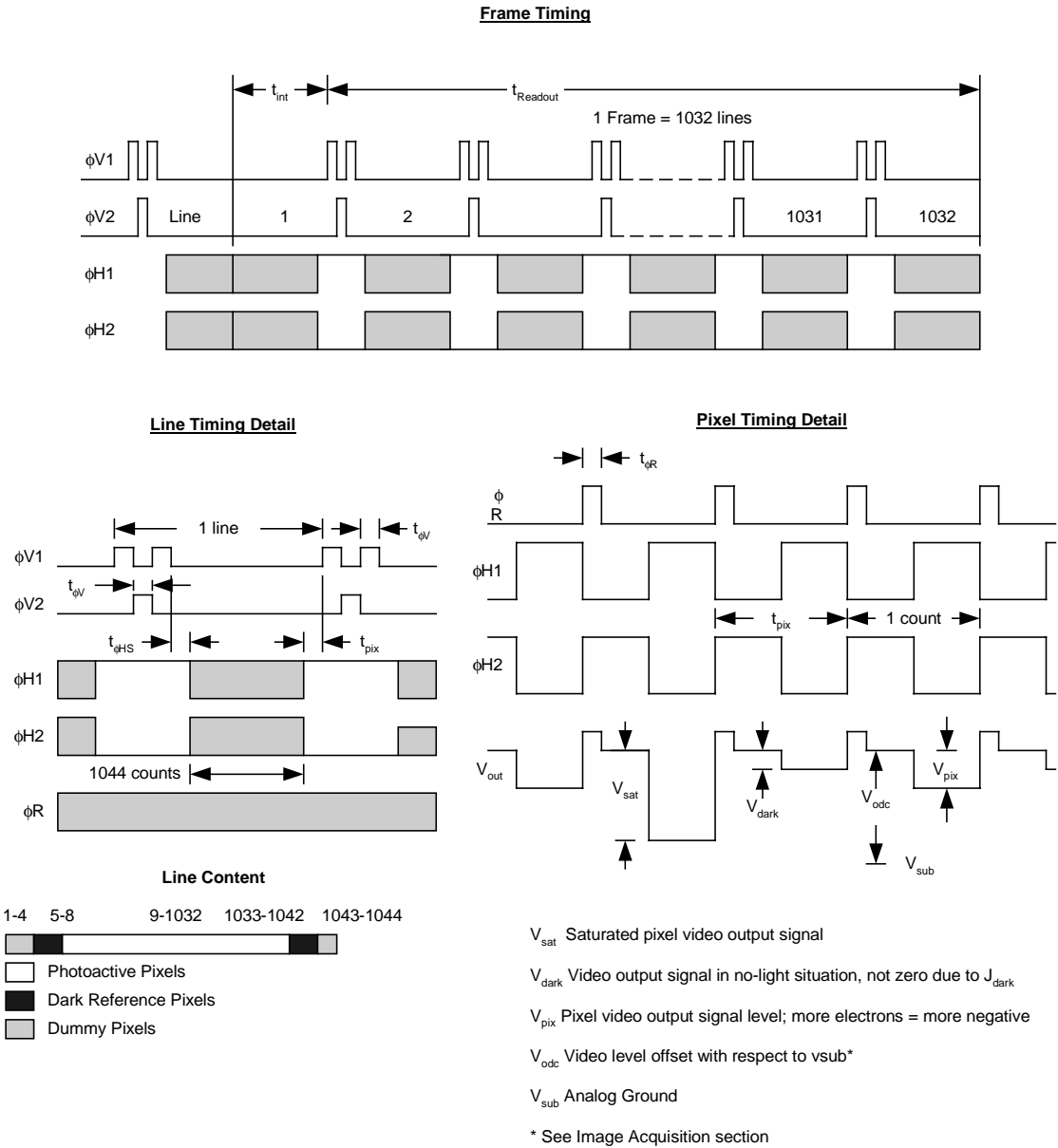
Figure 4 - Timing Diagram
