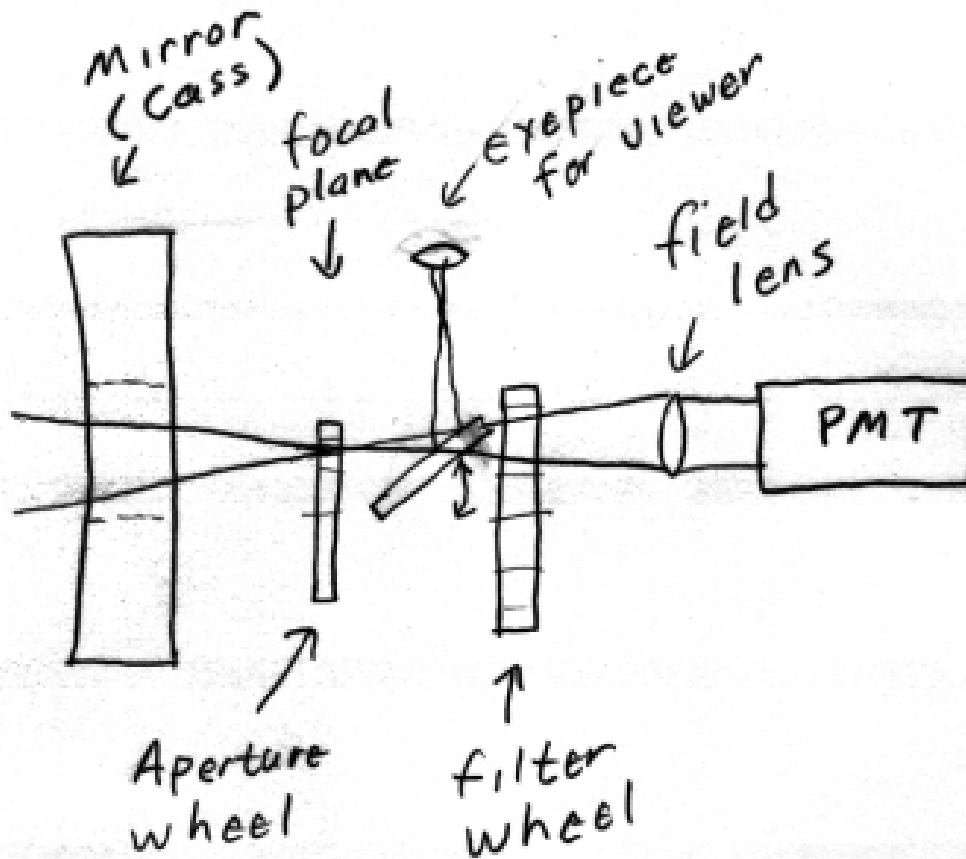
Figure 11.3: Schematic diagram of a simple photometer. The aperture wheel contains holes of various sizes that define the angular size of the spot in the focal plane which is measured by the photometer. Behind the aperture wheel is a mirror that can be flipped into the light path to direct light to an eyepiece. This “behind the aperture viewer” allows the astronomer to visually center the star in the aperture. The mirror is flipped down to allow light to pass to the detector. The filter wheel holds various filters that define the passband measured by the PMT. The field lens directs the light to the photocathode of the PMT. The PMT is usually cooled by dry ice (solid carbon dioxide).
