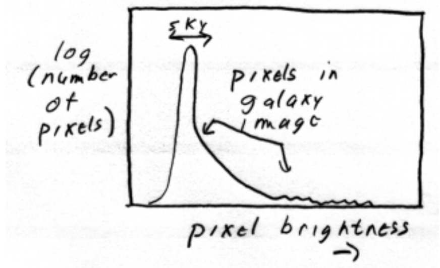
Figure 16.2: Histogram of a field largely filled with image of a galaxy. The galaxy pixels cover a smaller range of intensity than the star images, but a greater area of the chip. Many pixels in the outer parts of the galaxy are only a little above sky, so that the galaxy pixels blend into the sky pixels in the histogram.
