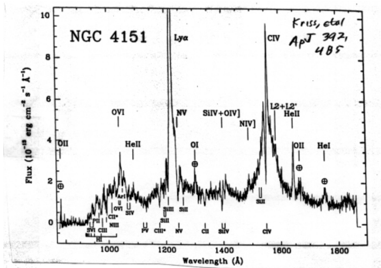
Figure 3.1: Example spectrum of an astronomical object, the active nucleus in galaxy NGC 4151. Note the units on the y axis ( 10^{-13} erg \text{s}^{-1} \text{cm}^{-2} \text{\AA}^{-1} ). Note the range of units on the x axis- this spectrum was obviously not taken with a groundbased telescope!
