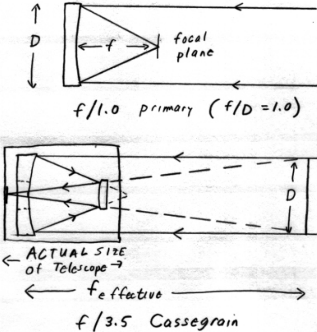
Figure 5.4: Effective focal length of a Cassegrain system. Top: Fast primary, with f=D ( f/1.0 ). Bottom: The effective focal length of the telescope is f=3.5 D ( f/3.5 ), but the actual length of the telescope is roughly f=D .
