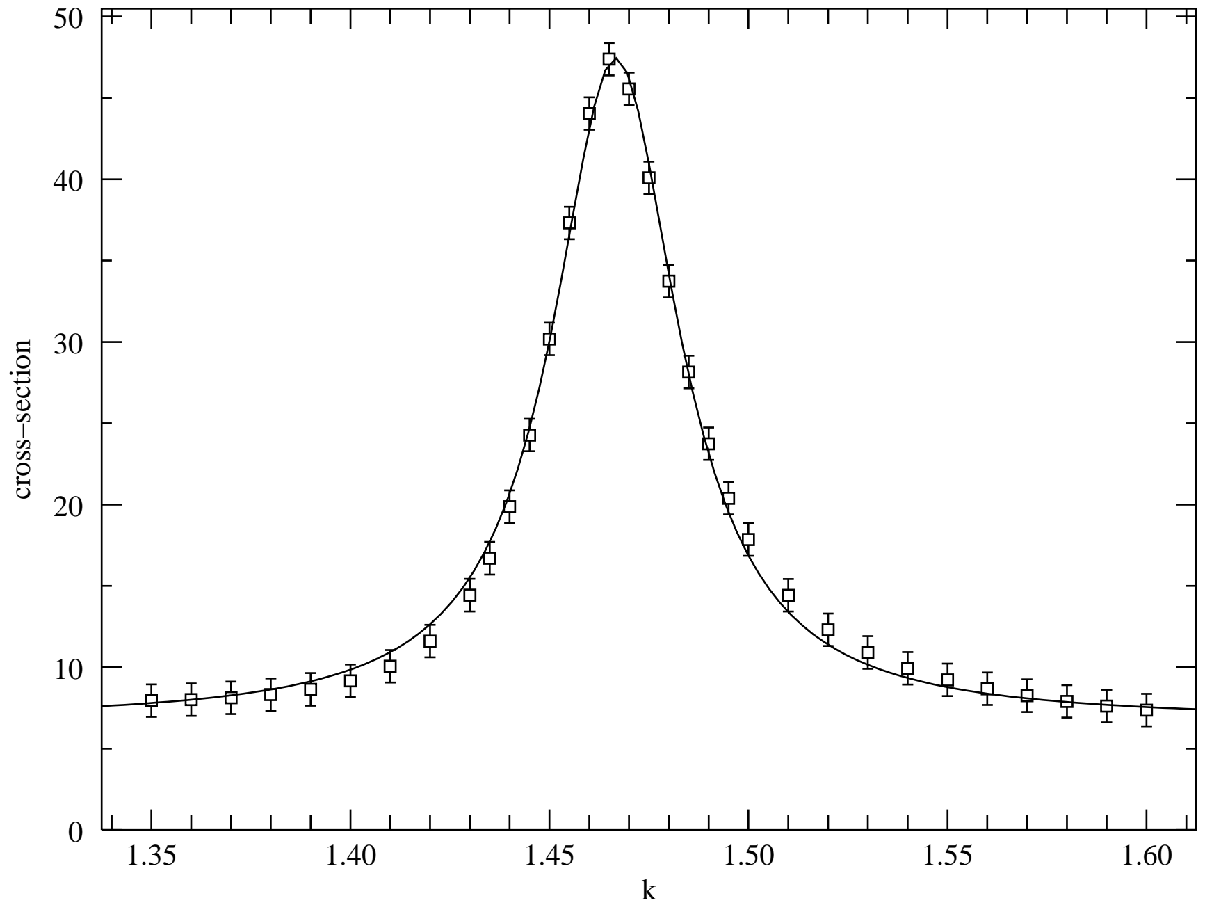
Breit-Wigner Cross-Section Fit
